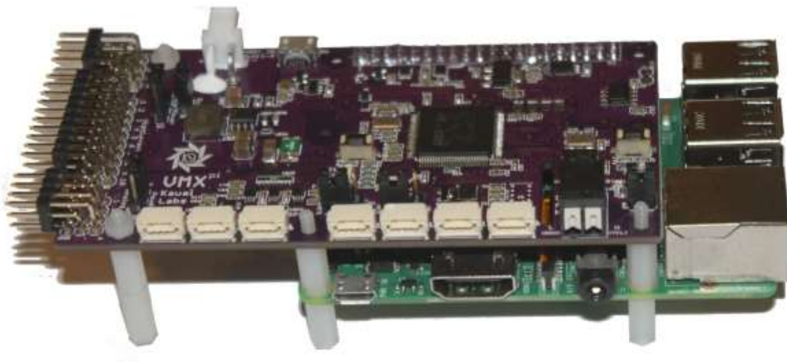
Figure 1 VMX-pi configured with Raspberry Pi 3
