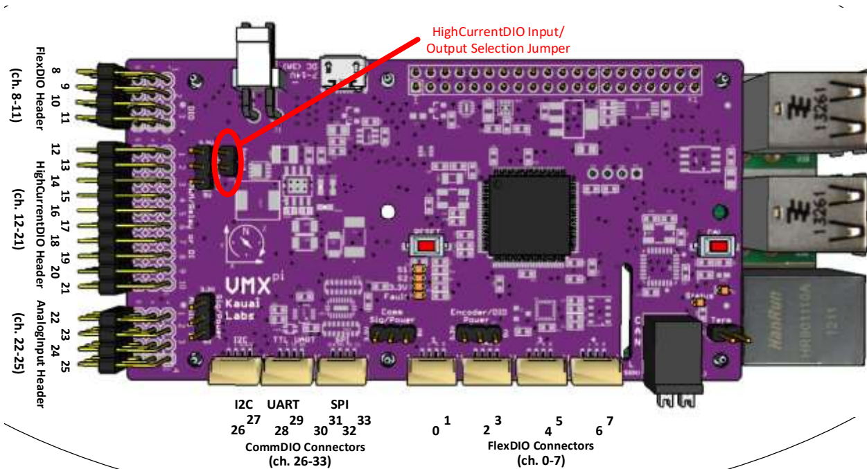
Figure 4 VMX-pi Channel Types and Numbers
