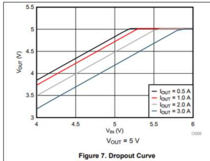
Figure 5 VMX-pi power supply voltage regulator dropout curve
