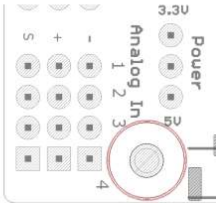
Figure 10 Analog Input Header (VMX Channels 22-25) pinout
